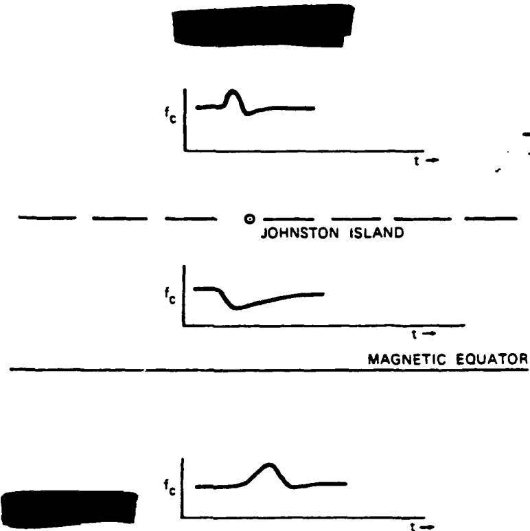
FIGURE 3-23 [REDACTED] GEOMAGNETIC FIELD DEPENDENCE OF ACOUSTIC-GRAVITY WAVE
